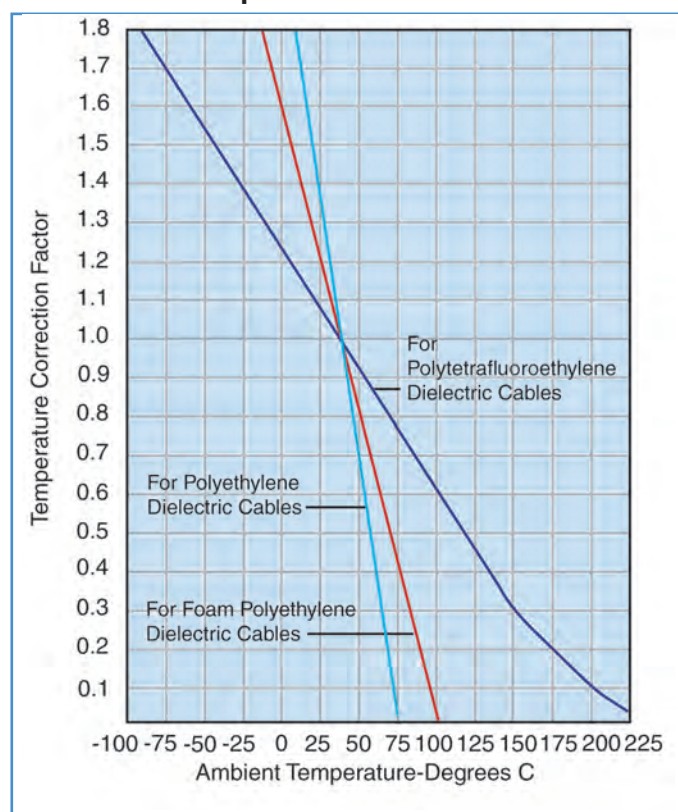
Fig. 6 Power Temperature Correction Factor
