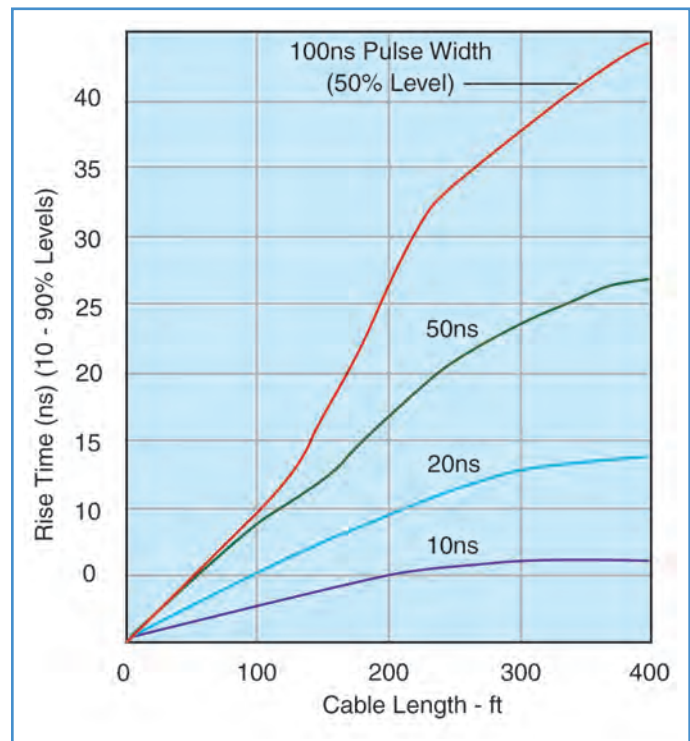
Fig. 11 Pulse Distortion
