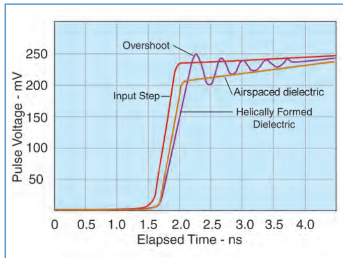
Fig. 13 Step Response (Output Amplitude vs. Time)
